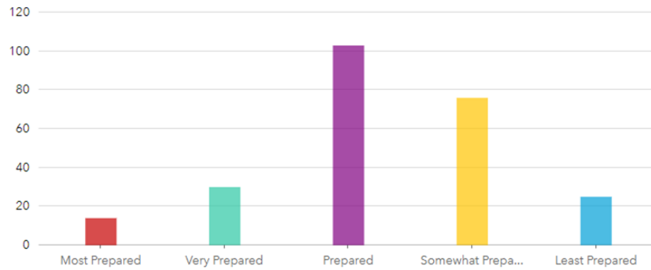
c. Earthquake
